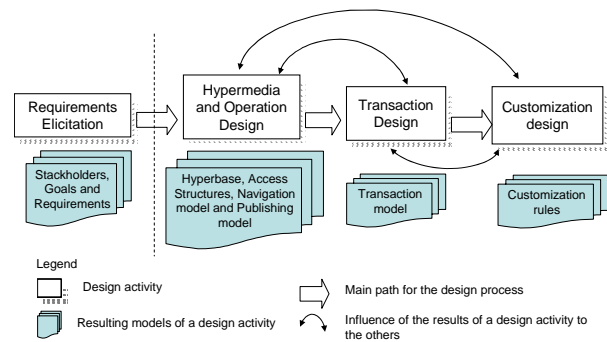
Figure 1. The UWA Web application design process.
